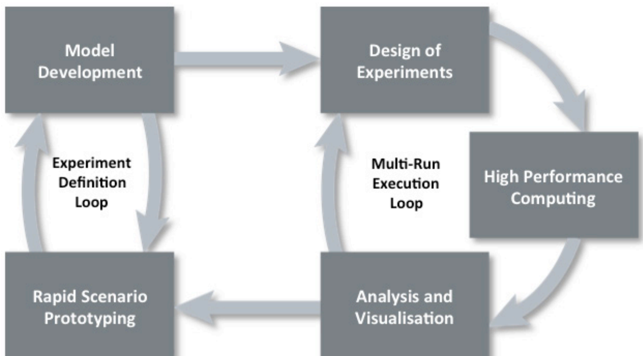
Figure 1. Data Farming “Loop of Loops”
